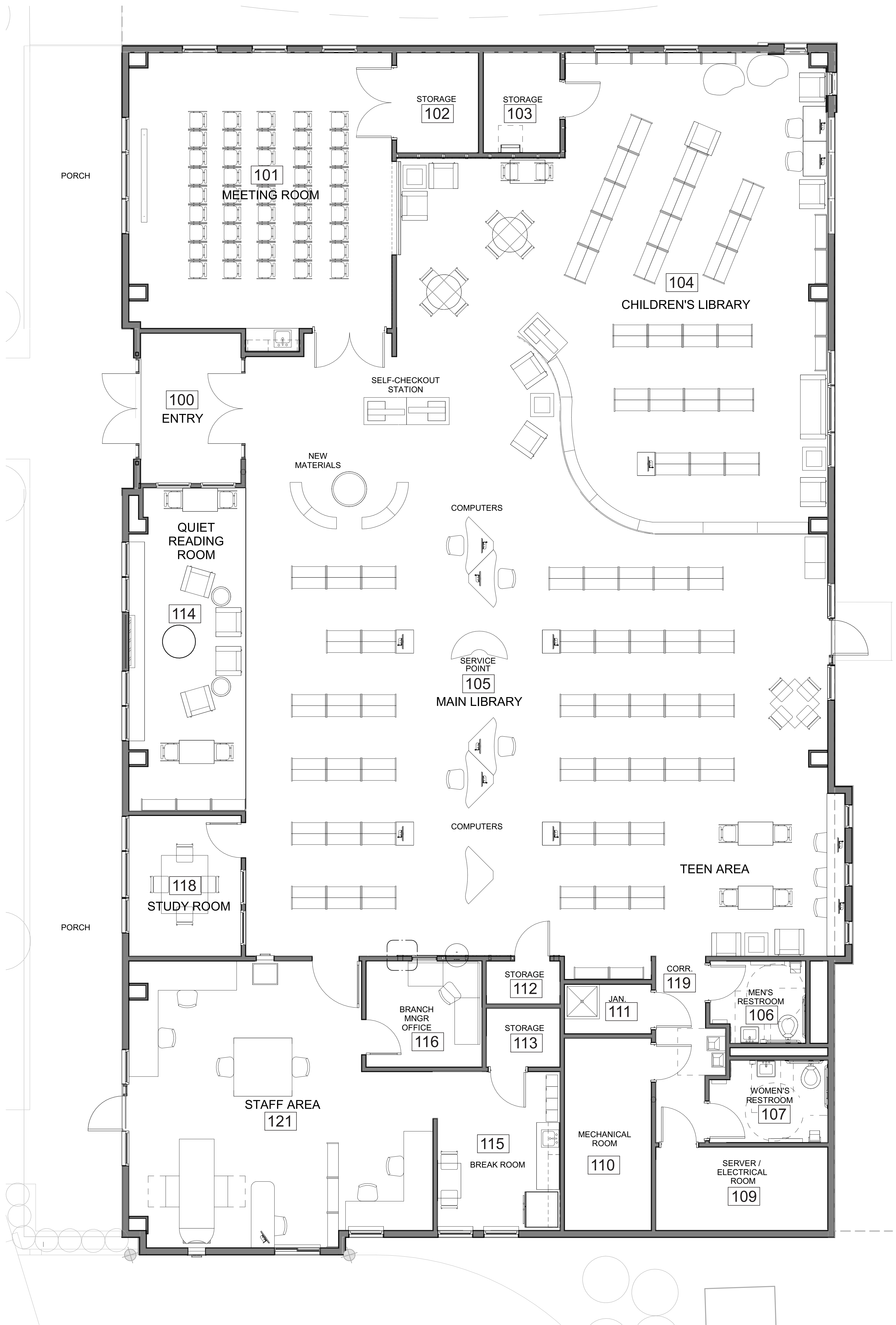
1 First Floor Plan 1/4" = 1'-0"
